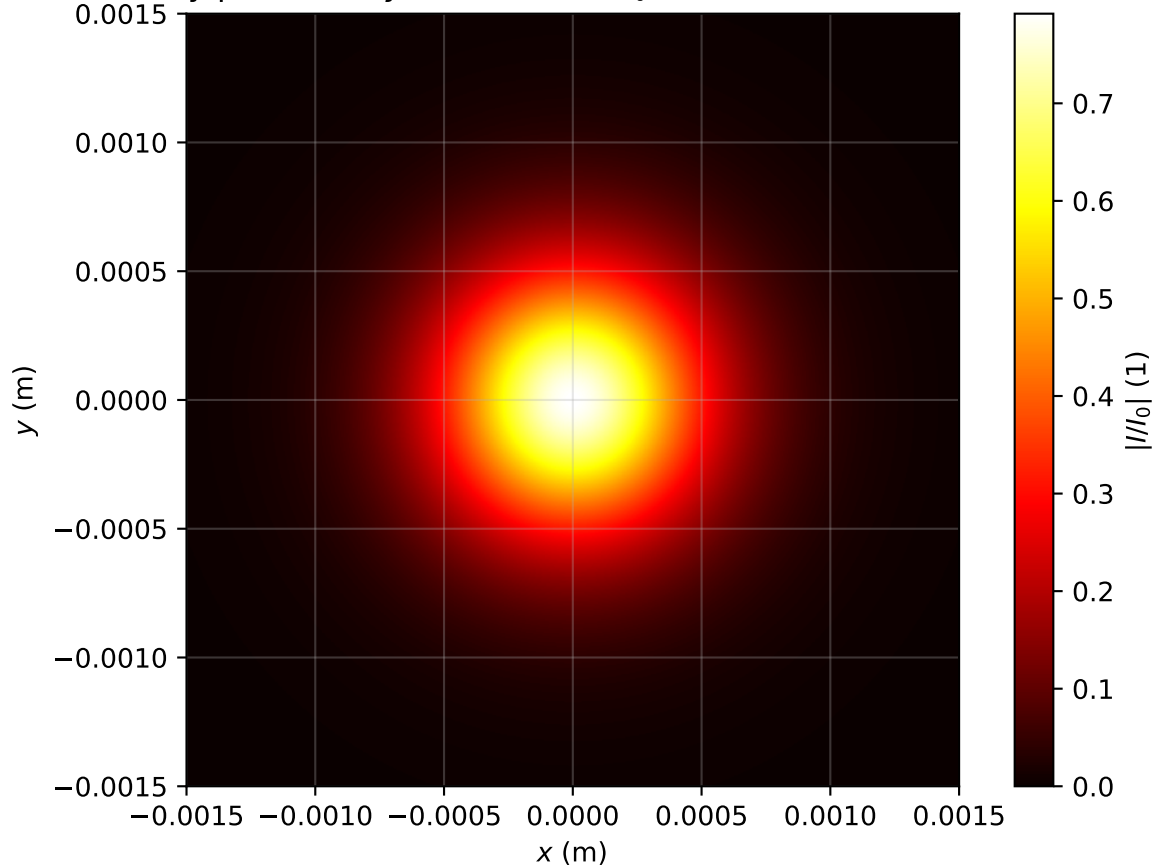
Intensity profile I(x, y, z = 2.548m)/I_0 , \text{Pin}=0.6\text{Pcr} , artificial time
